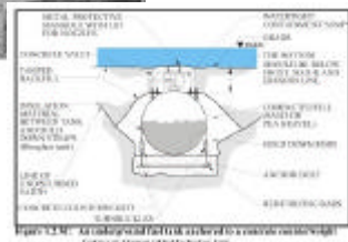
Figure 3.2.3B: An anchoring detail for a tank attached to a concrete structure
